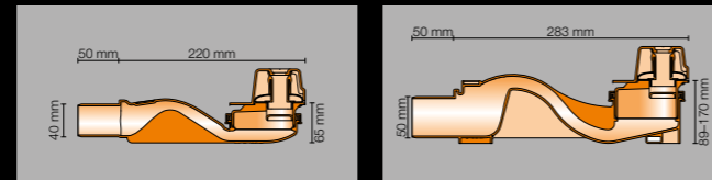
Schlüter-KERDI-LINE-VARIO-H 40
